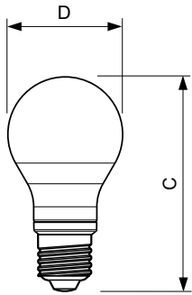
Bulb A60 220~240V 5W 470lm 2700K E27 D
